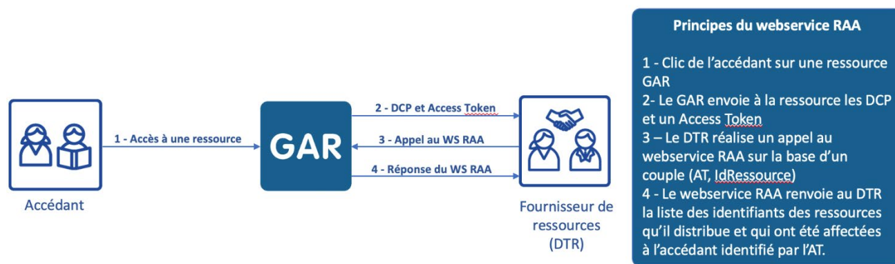
Figure 24 - Principe du webservice RAA
